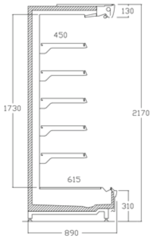
MERGA 89 X 217
