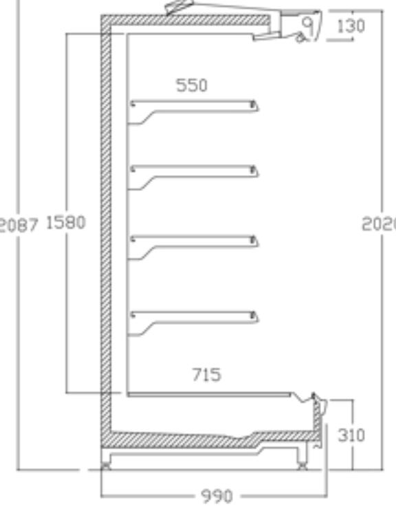
MERGA-F 99 X 202
