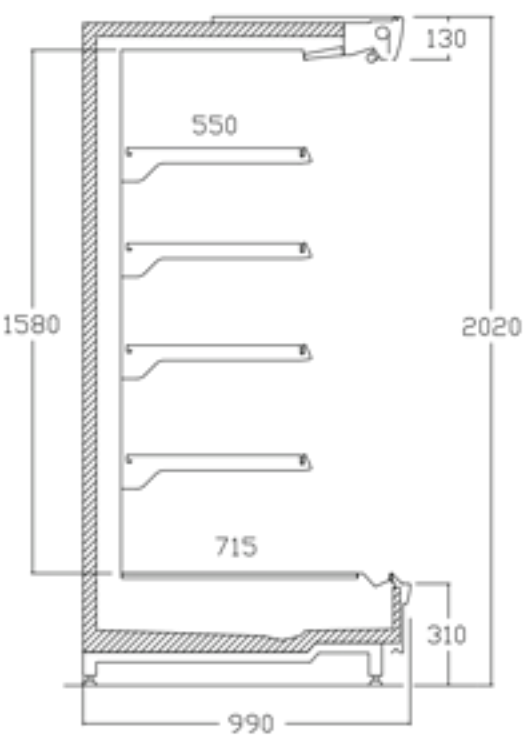
MERGA 99 X 202
