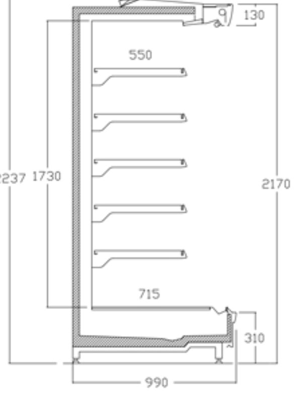
MERGA-F 99 X 217
