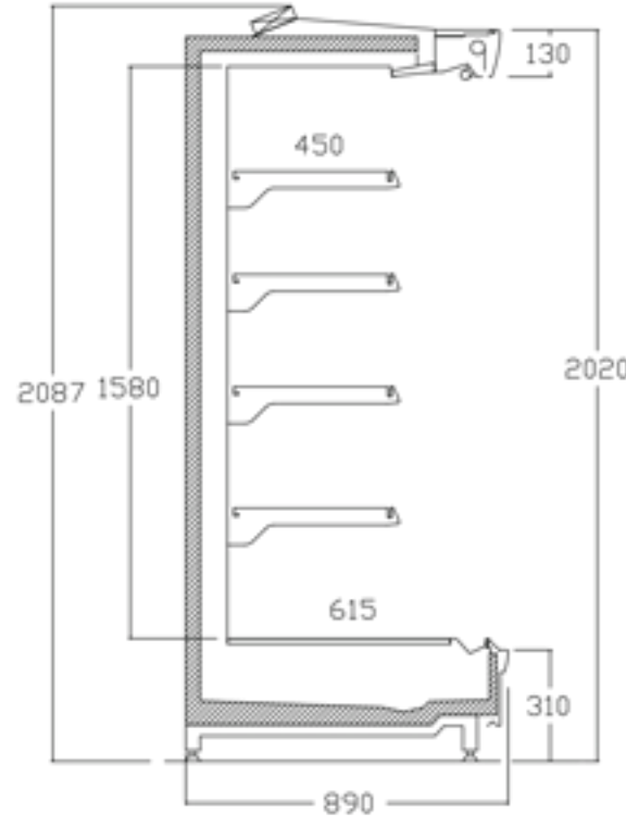
MERGA-F 89 X 202
