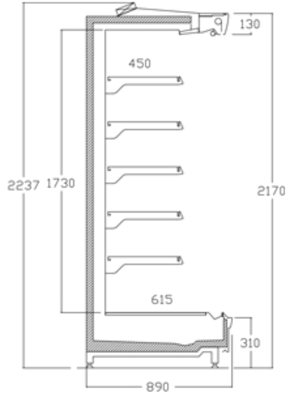
MERGA-F 89 X 217
