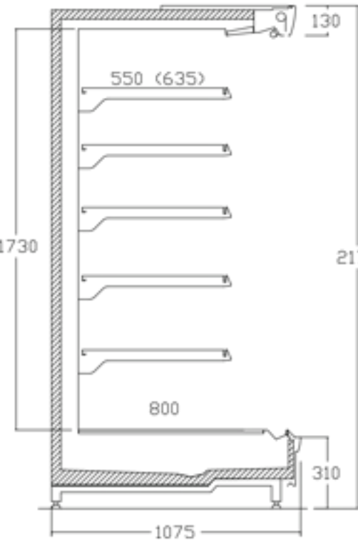
MERGA 107 X 217
