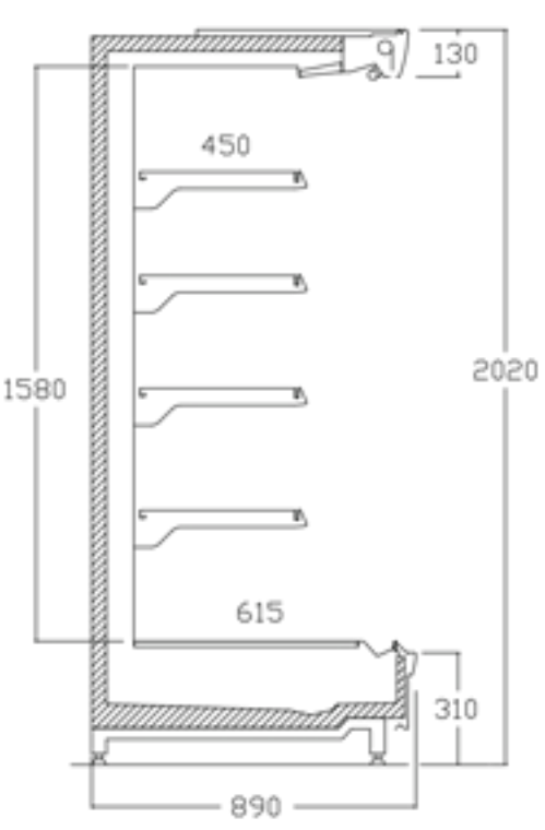
MERGA 89 X 202
