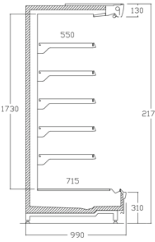
MERGA 99 X 217
